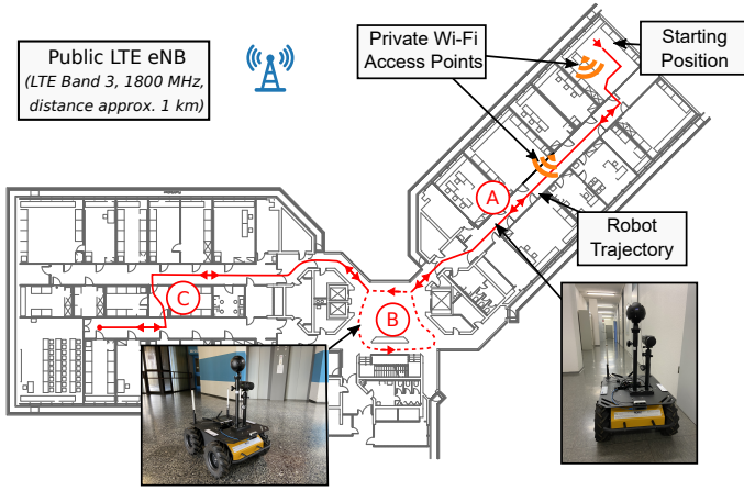
Fig. 7. Trajectory of the robot during the experiments in the challenging indoor scenario. Especially in the stairwell area (B) a lot of shadowing and negative interferences occur due to the building's concrete walls. The Wi-Fi access points are located inside the building, while the public LTE cell tower is on the rooftop of a close building in an approximate distance up to 1 km. Area (A) is covered by Wi-Fi, in (B) signal strength is decreased, while in area (C) only the LTE signal is available.
